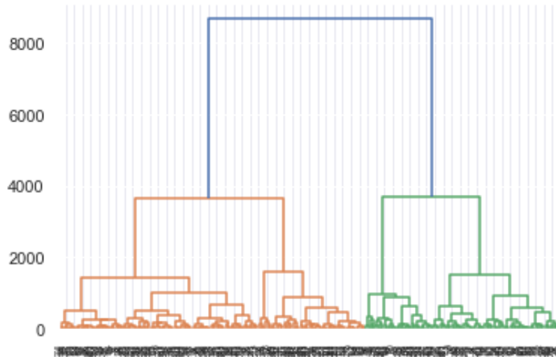
Figure 7.6: Dendrogram for the complete dataset.
